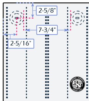
14164F-MMH Interior Structured Wiring
